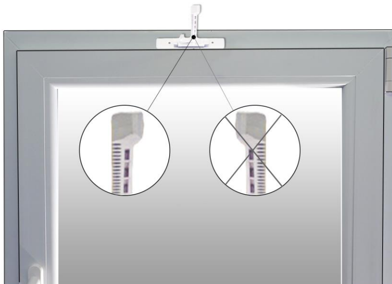
Figure #3C: SMARWI holder stuck in the middle of the window frame, tightly above the upper edge of the inner frame. The orientation of ridge teeth always on the left
